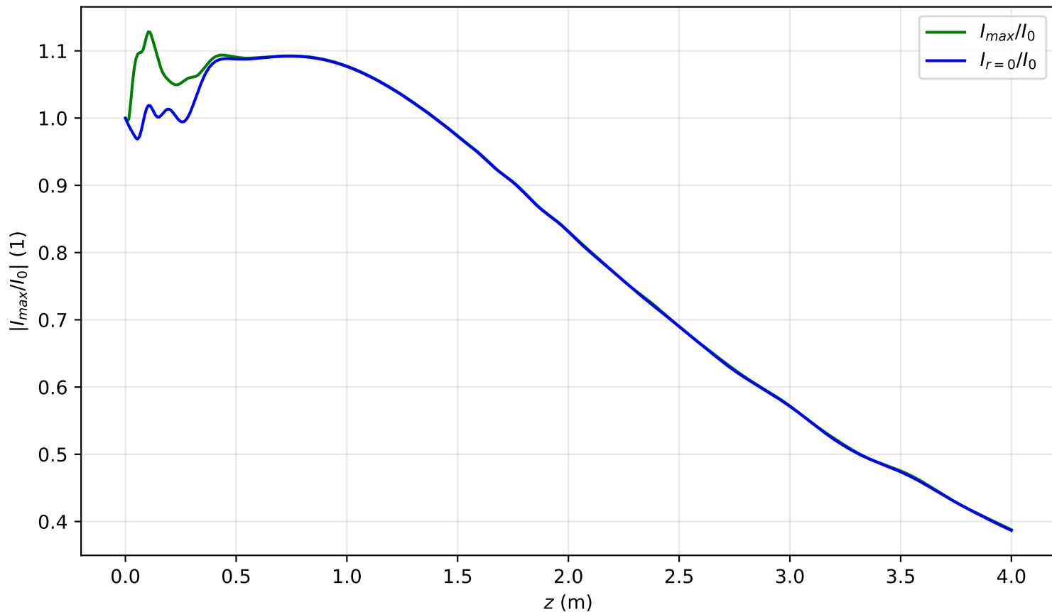
I_{max}(x = 0, y = 0, z)/I_0 , P_{in}=0.5P_{cr} , noisy input, artificial time
